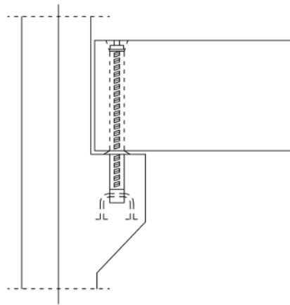
Figure 3.1. Beam-Column connection
